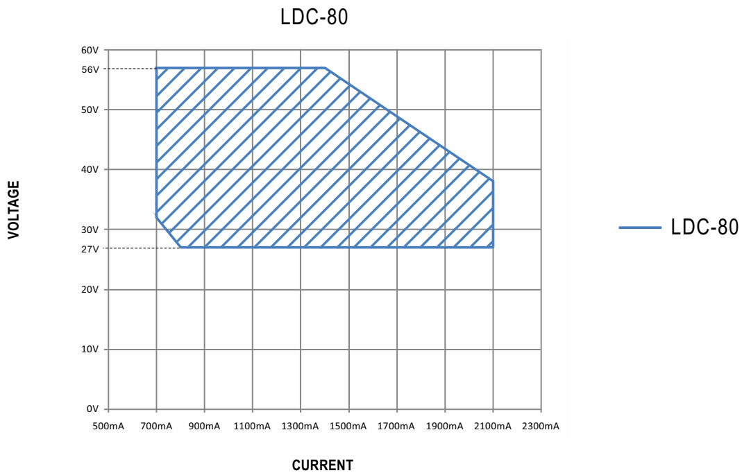
◎ Rated current setting table
